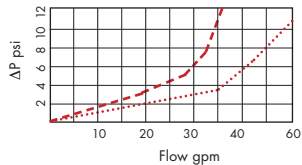
\Delta P PF9 & PF20 Housing*
