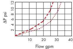
\Delta P PF9 & PF20 Housing*
