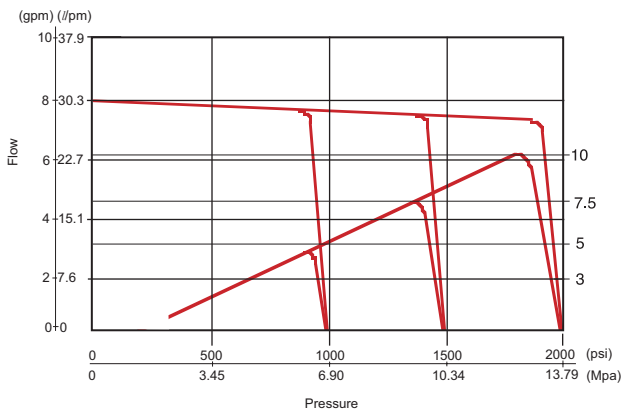
Typical performance curves based on ISO VG46 Oil @120°F, (49°C)
