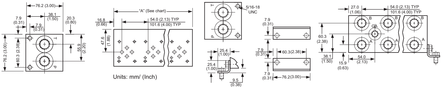
D03 & D05 Series- Industry Standard Manifolds
