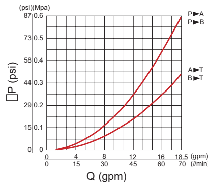
D05 Pressure Drops
