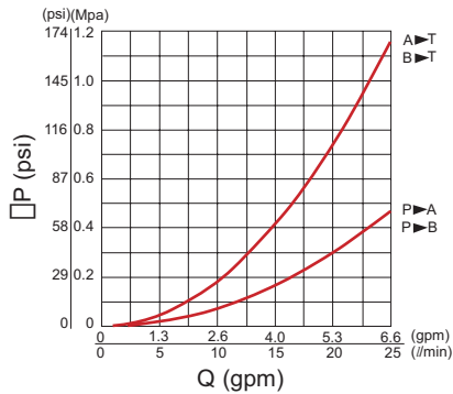
D03 Pressure Drops
